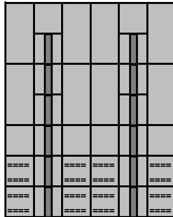
DPWC-133 6 X 7 Double PWC Dry Dock (for 1 & 2 Seaters)
